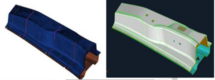
3D FE and CAD models
